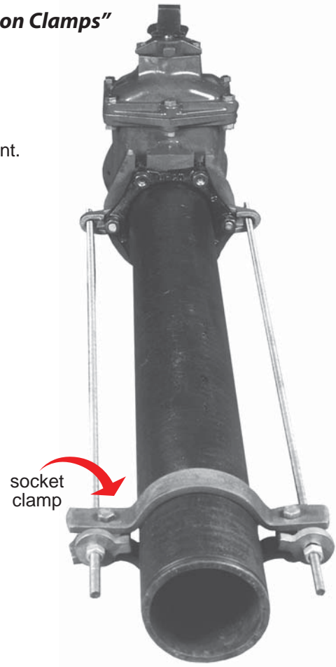
Typical Installation
