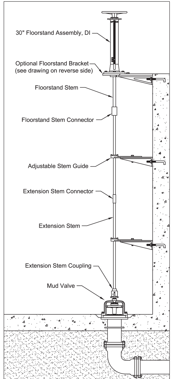
Typical Floorstand installation
