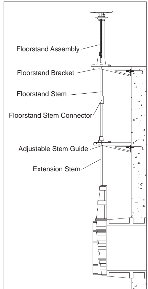
Typical Stem Guide installation
