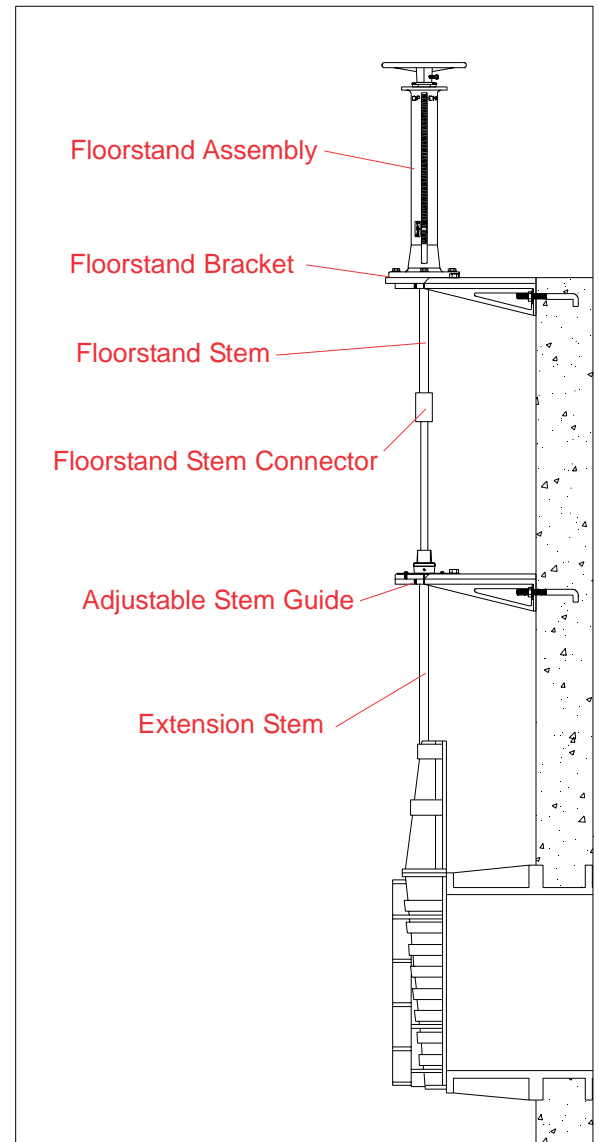
Typical Stem Guide installation.
