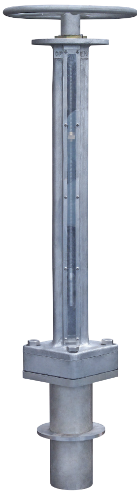
Sealed Assembly For use with hazardous gasses. Variety of sealing materials are available.
