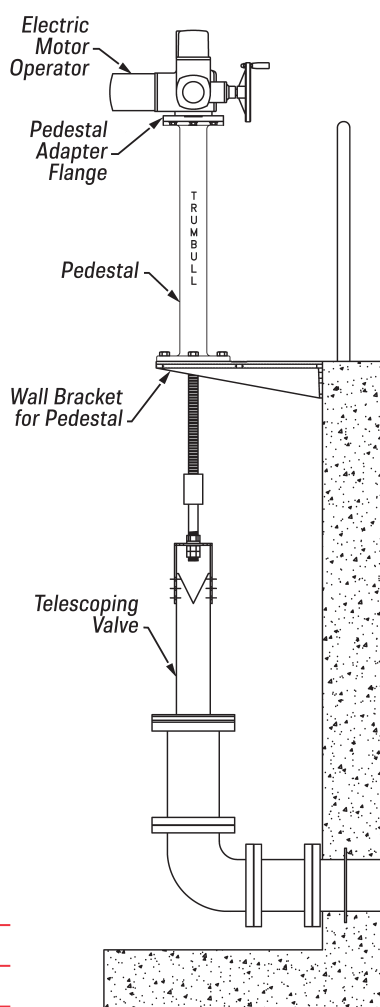
Typical installation
