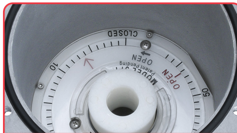
POSITION INDICATOR
