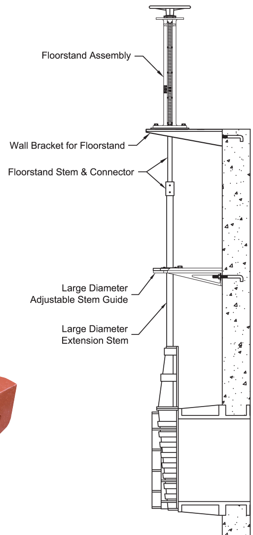
Typical installation
