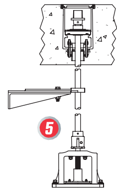
4 Floor Box with Position Indicator
