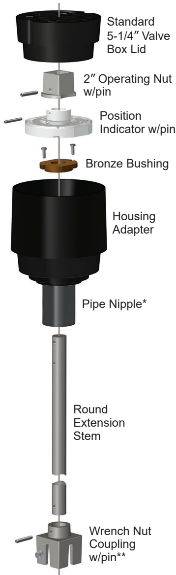
ROUND EXTENSION STEM
